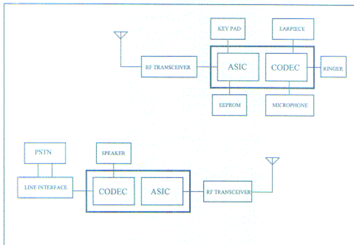
HD-950 System Architecture
