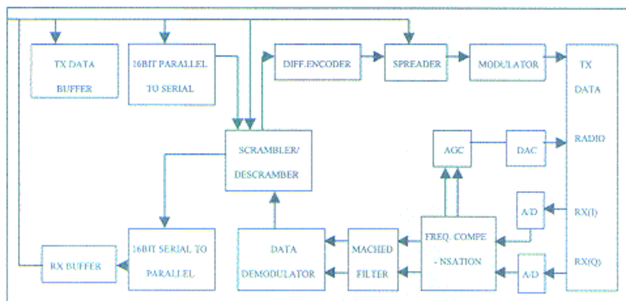
DCT Spread Spectrum Engine Block Diagram
