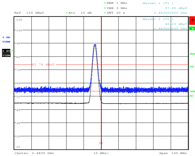
Figure 19: Radiated Emissions at Band Edge, Spectral Diagram, Mode C (2480MHz) at 1.5m height
