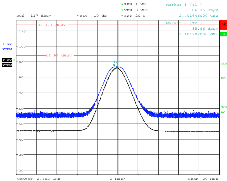
Figure 10: Field Strength of Fundamental, Spectral Diagram, Mode A (2402MHz) at 0.8m height
