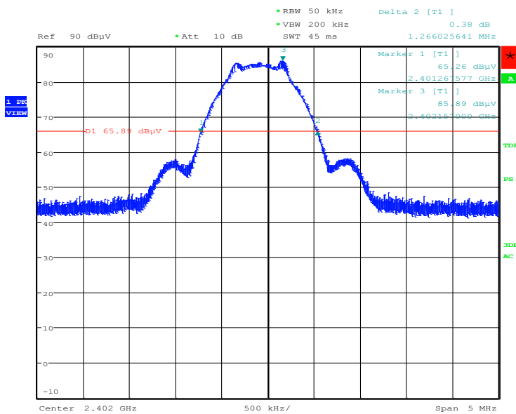
Figure 4: 20dB Bandwidth, Mode A (2402MHz)
