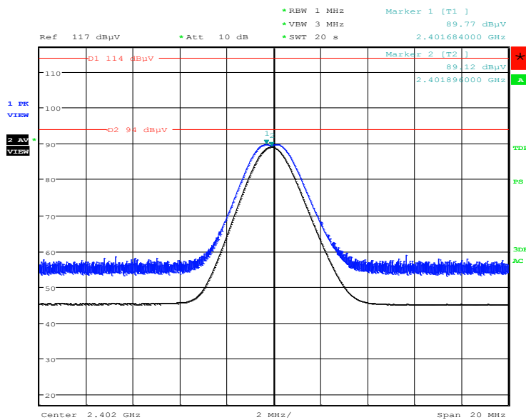
Figure 13: Field Strength of Fundamental, Spectral Diagram, Mode A (2402MHz) at 1.5m height
