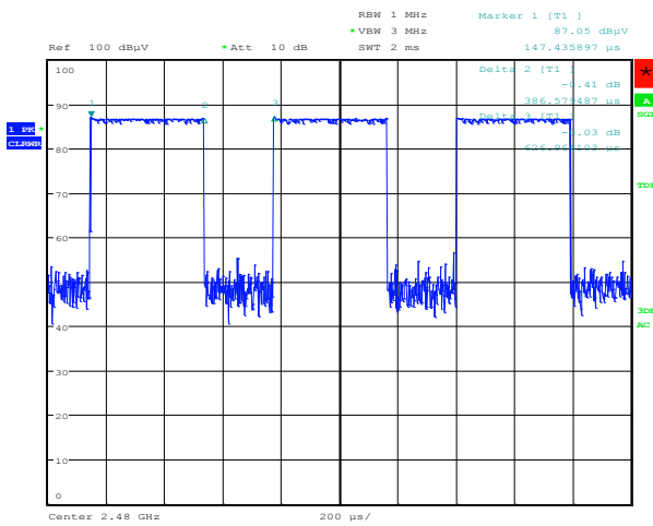
Figure 4: Duty Cycle, Mode C (2480MHz)
