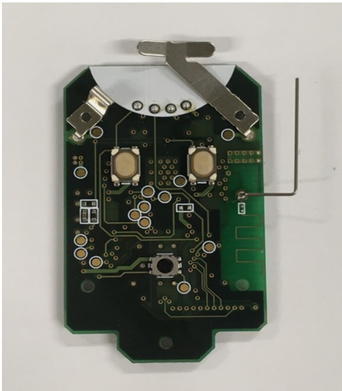
PCB side 1
