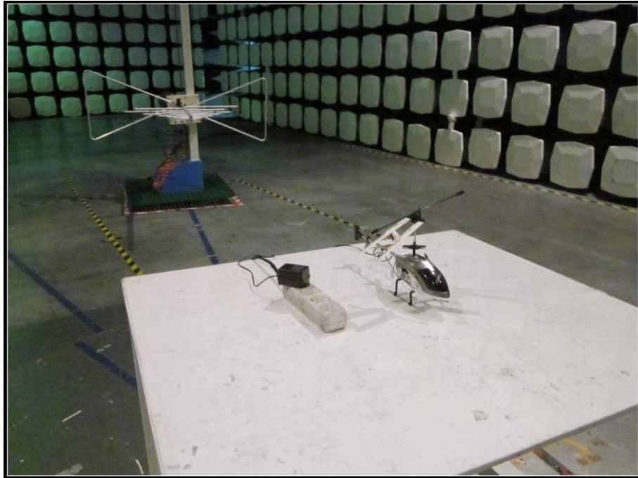
Charging mode
