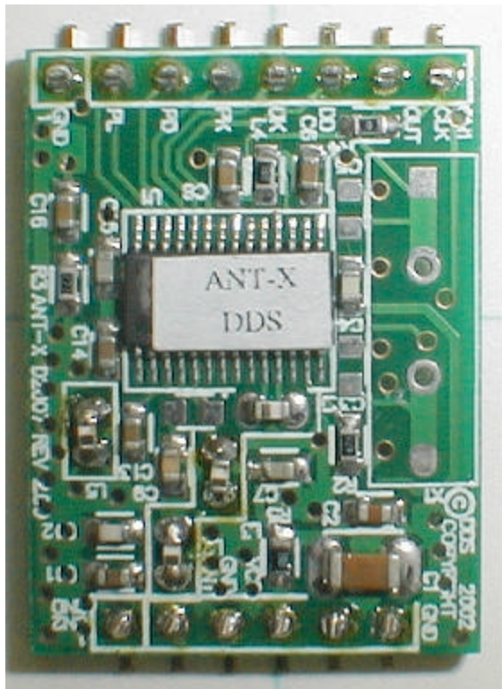
ANT Module, Top View
