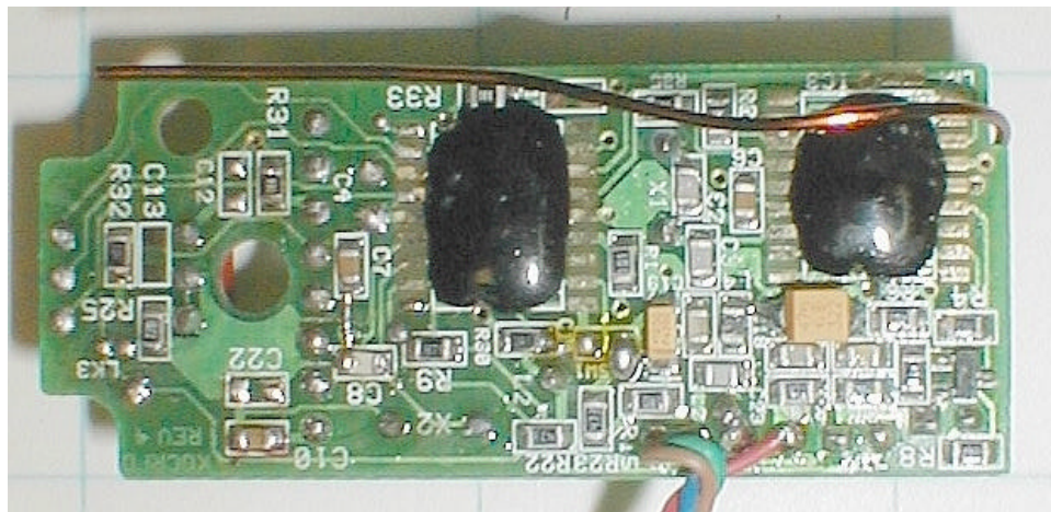
Functional PCB, Bottom
