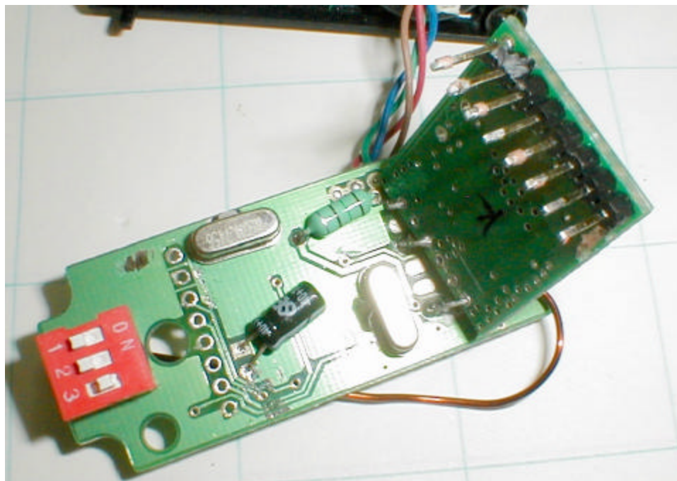
Function PCB Top; ANT Module Desoldered and Rotated
