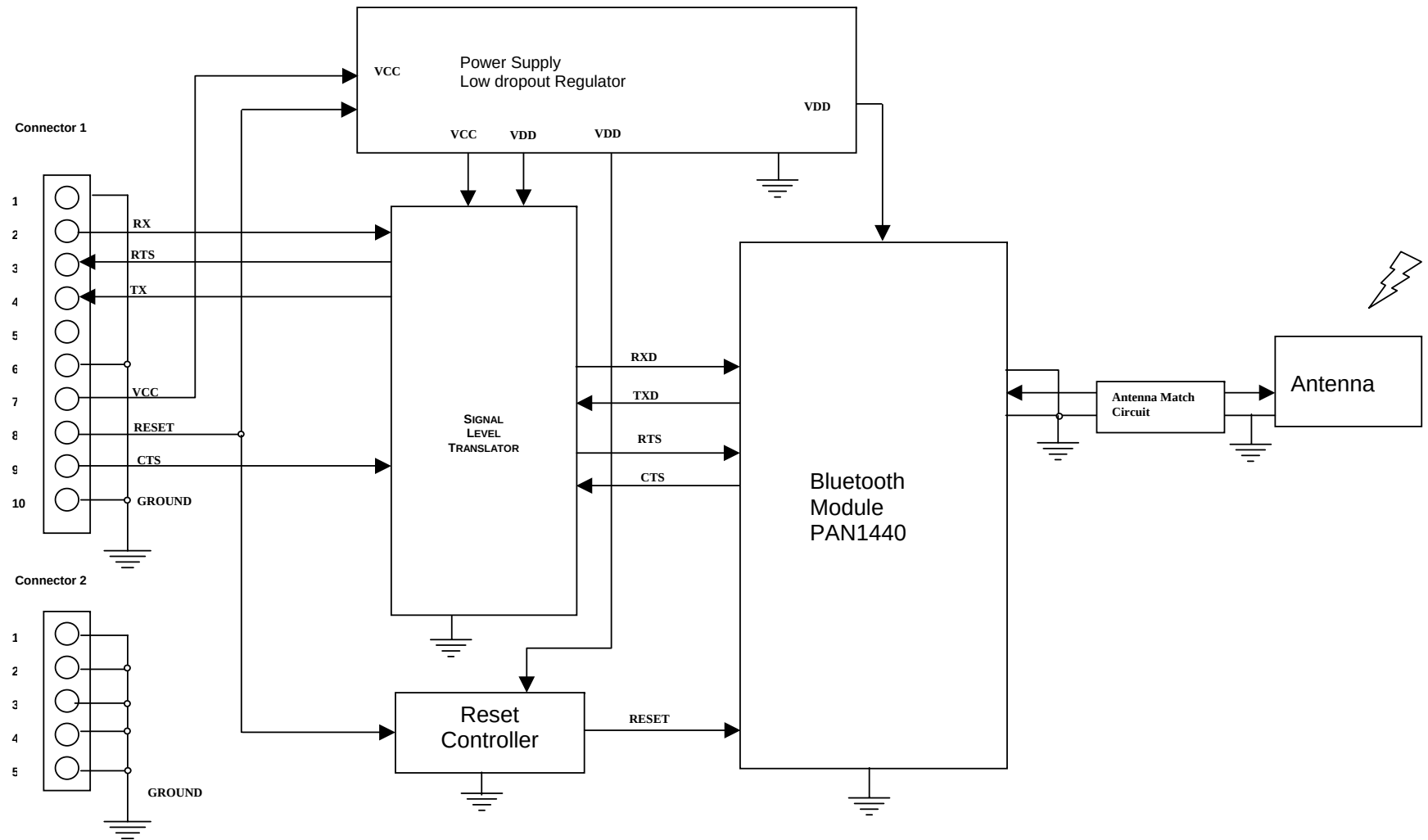
Fig. 7.2 - Block Diagram of Bluetooth transceiver
