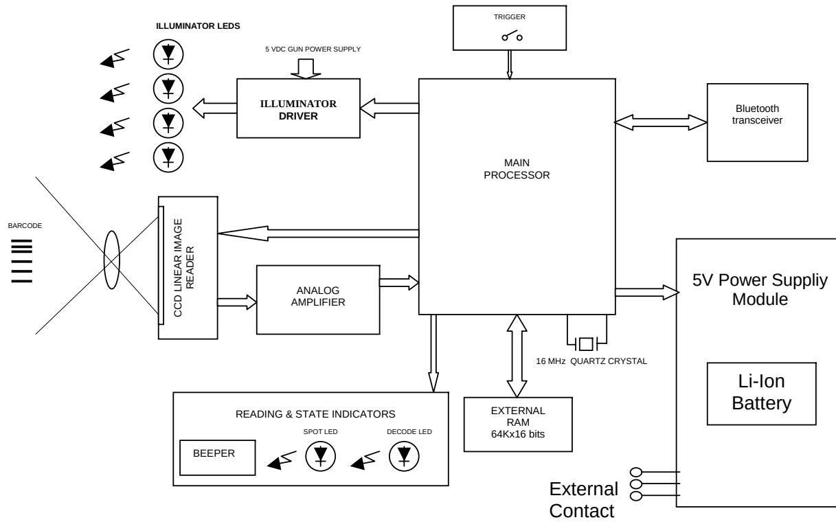
Fig.7.1 – Gryphon BT Block Diagram
