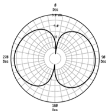
Free Space Elevation Pattern PHI=0
