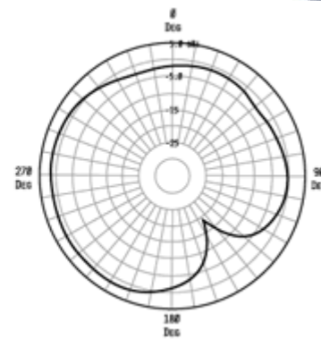
Free Space Elevation Pattern PHI=90
