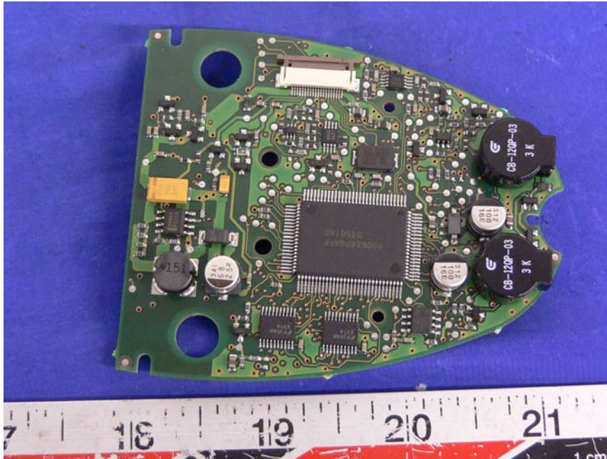
Handset – Board 1 Component View
