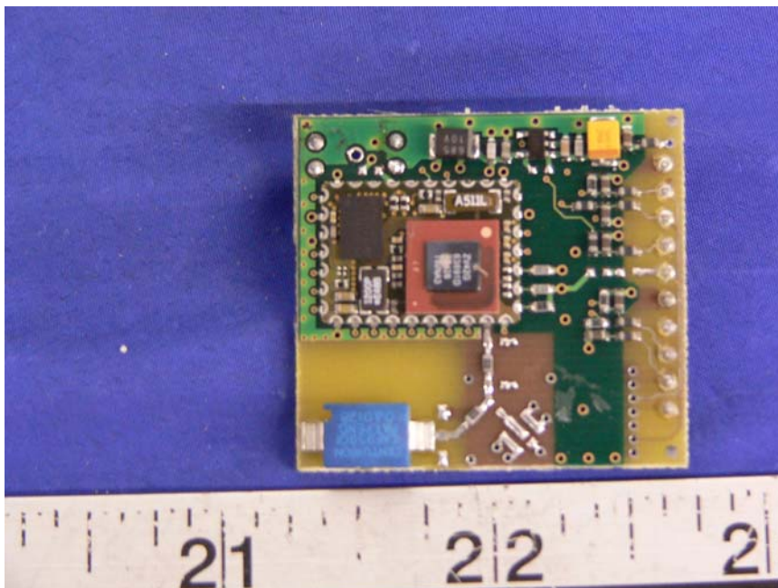
Base – Transmitter Component View
