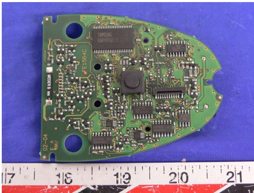
Handset – Board 1 Solder View
