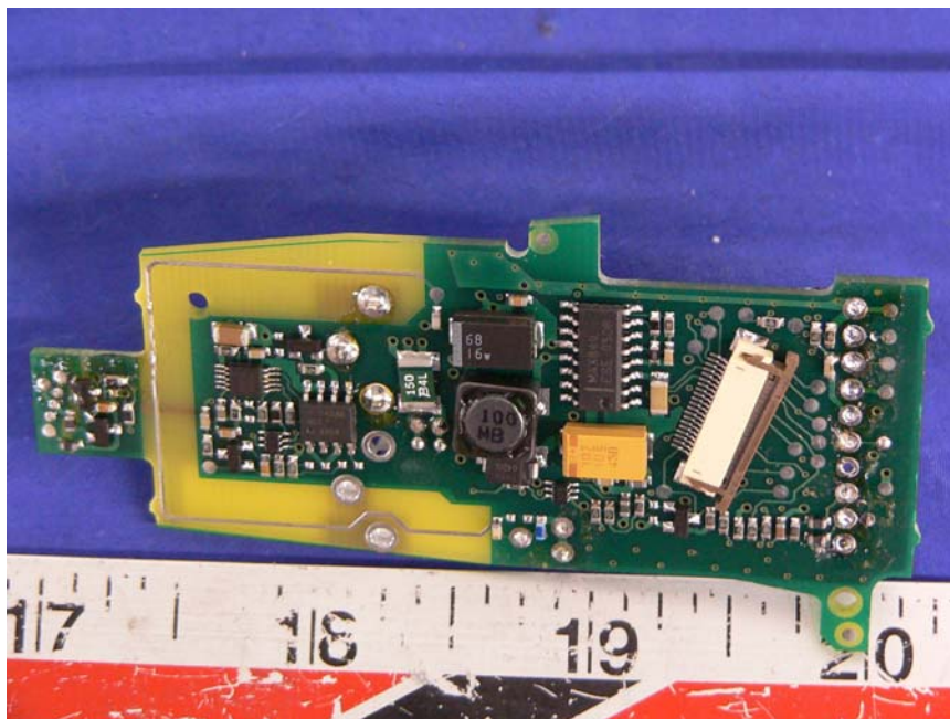
Handset – Board 2 Solder View
