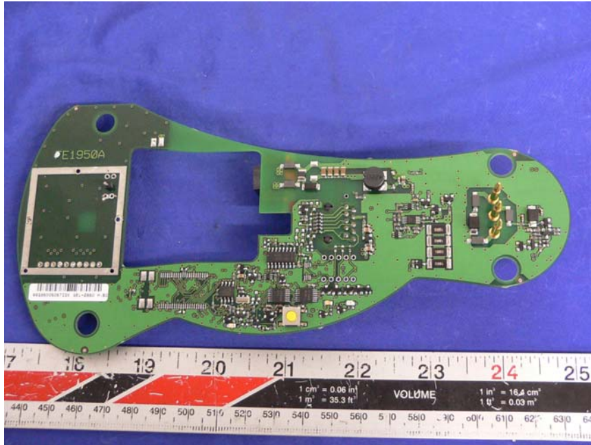
Base – Solder View
