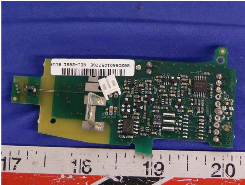
Handset – Board 2 Component View
