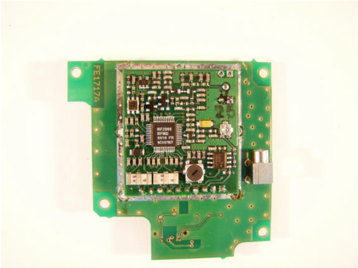
2371 RADIO BOARD PLUS RT14 TOP
