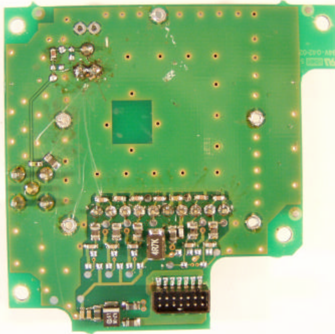
2371 RADIO BOARD BOTTOM
