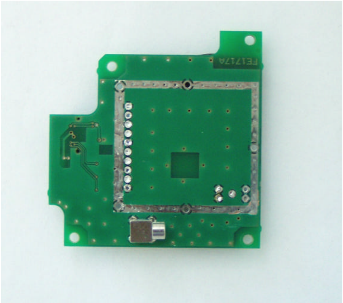
2371 RADIO BOARD TOP
