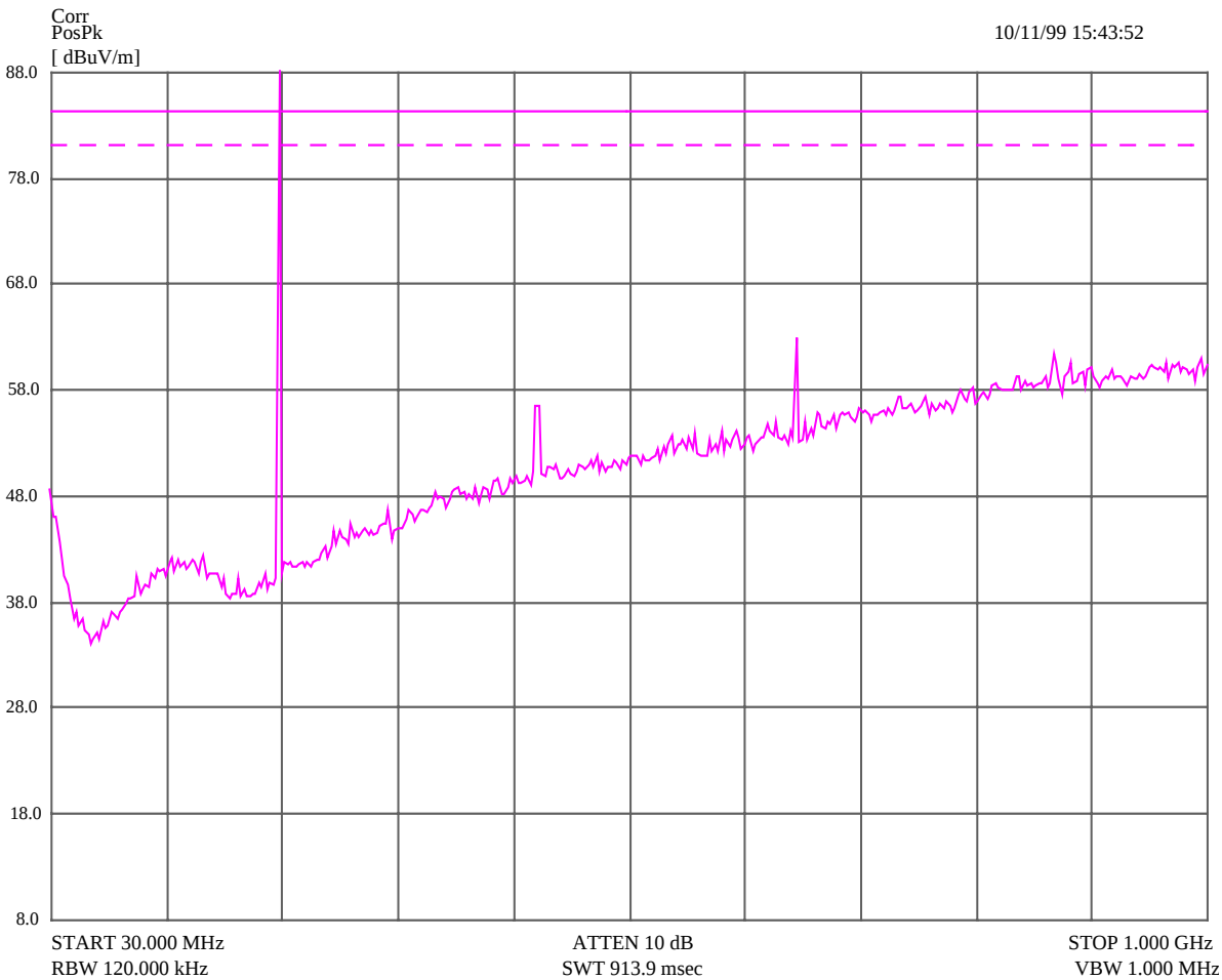
Receiver (Graphic) 1
