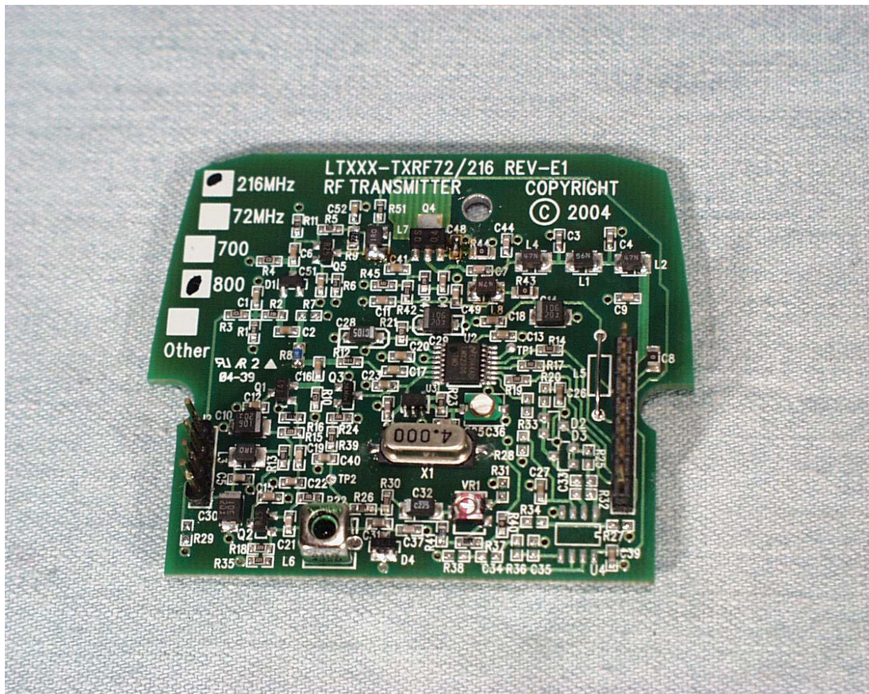
View of the Component Side of the Transmitter PCB
