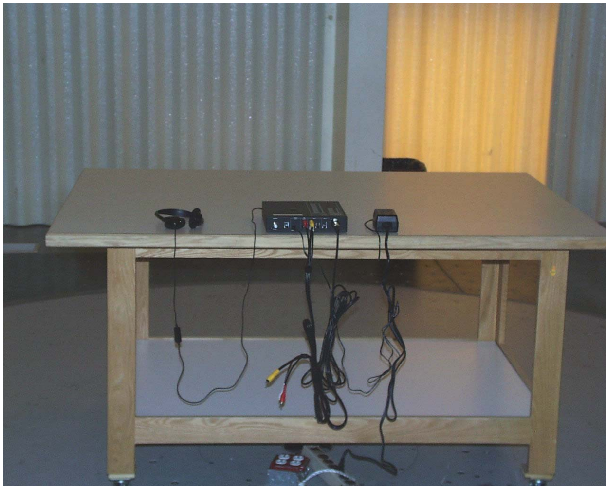
Back View Radiated Spurious Emission Configuration
