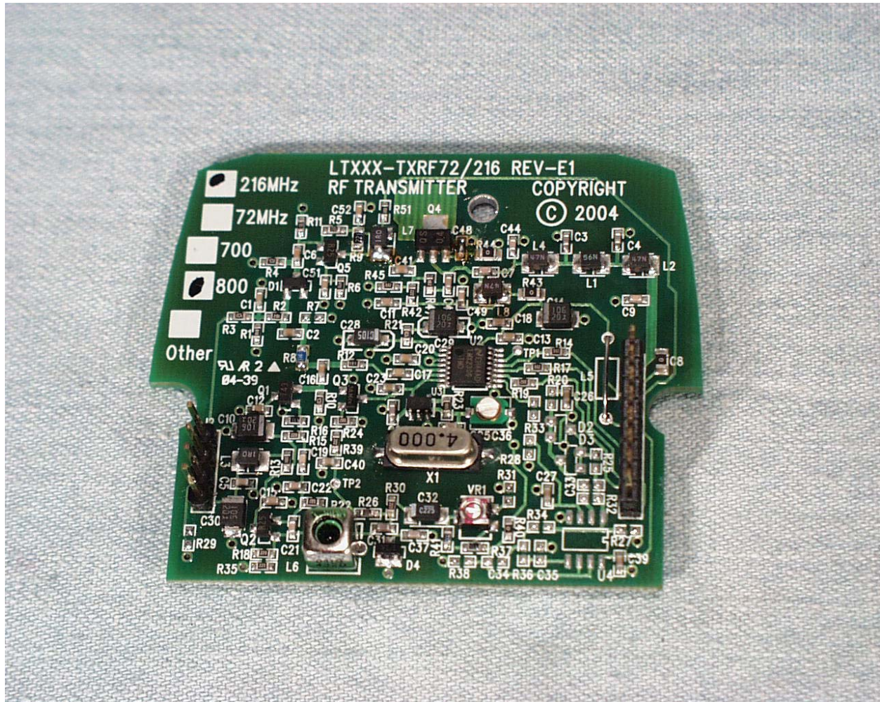
Photograph 6 - View of the Component Side of the Transmitter PCB
