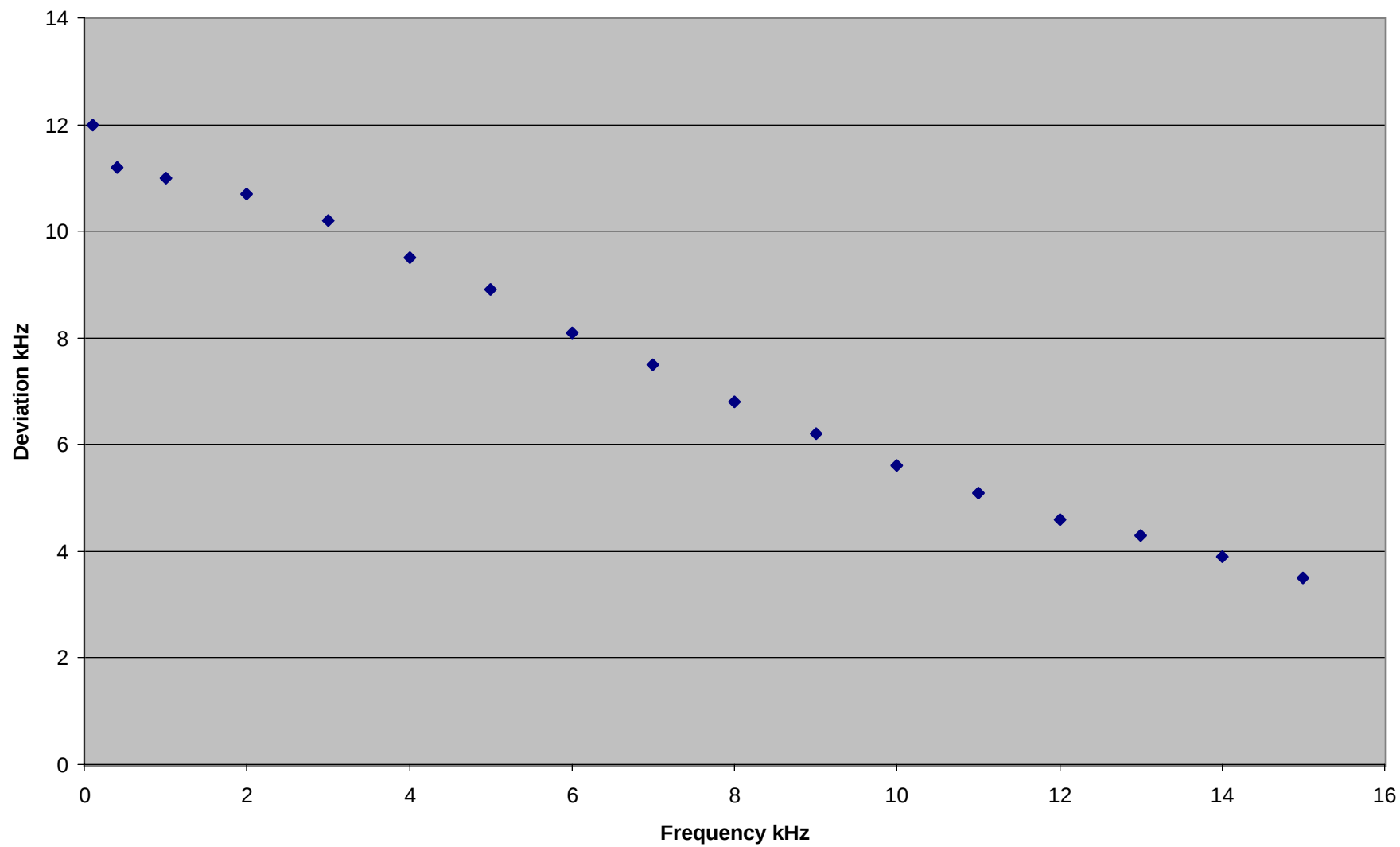
LT700 Frequency Response Ch. 2K
