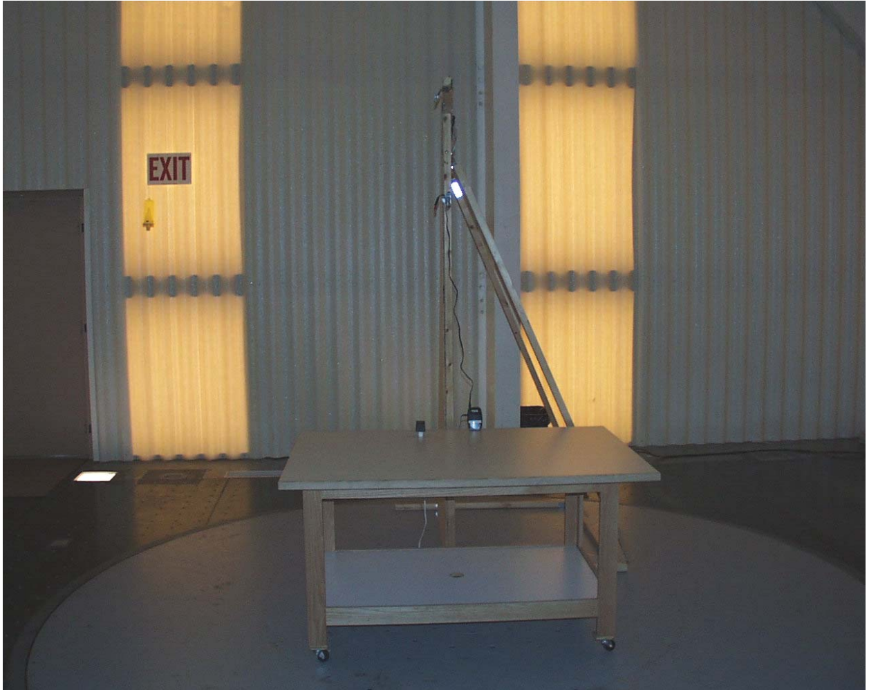
Front View Radiated Spurious Emission Configuration
