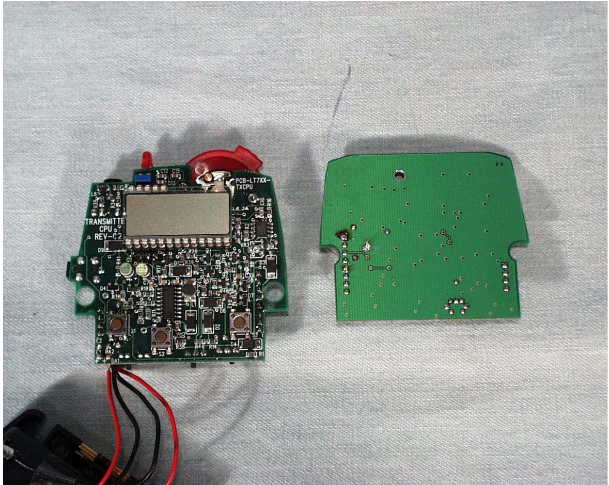
View of Side B of the PCB
