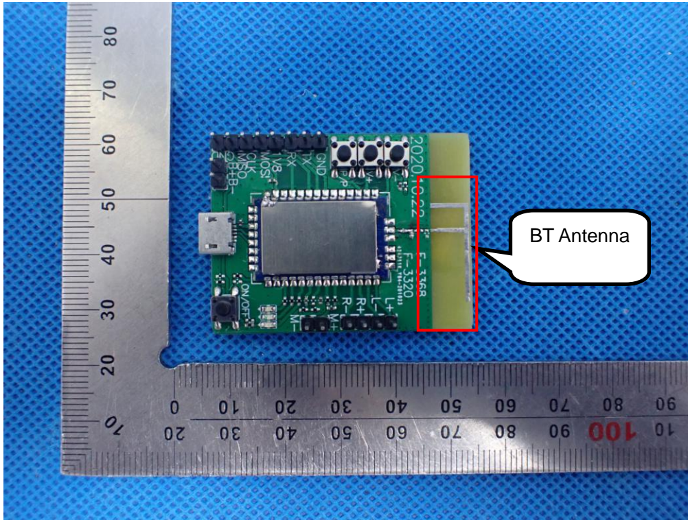
WHOLE VIEW-2 OF EUT
