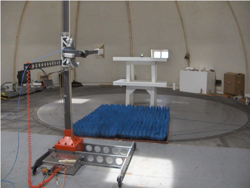
Emissions above 1 GHz
