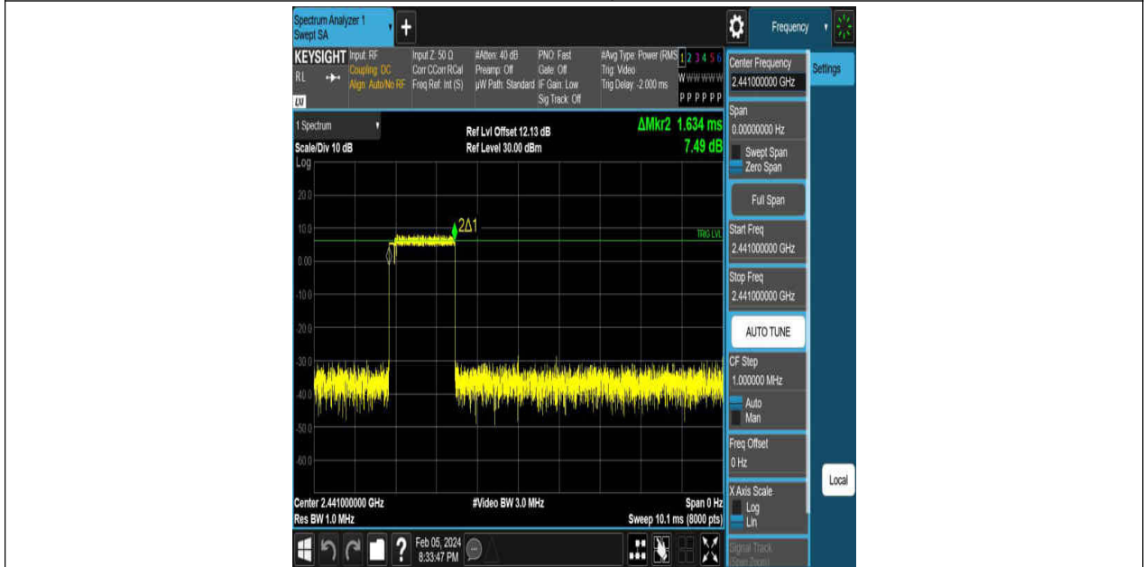
3DH3-Ant1-Hop-PASS
