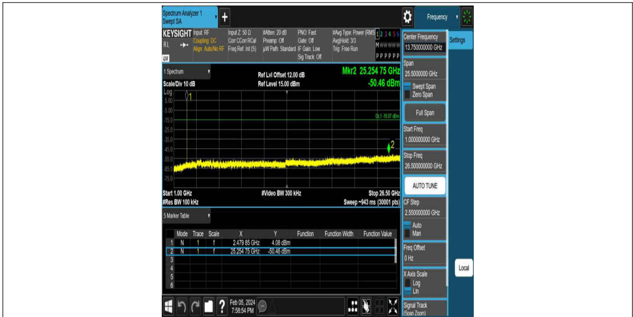
DH5-Ant1-2480-1000~26500-PASS
