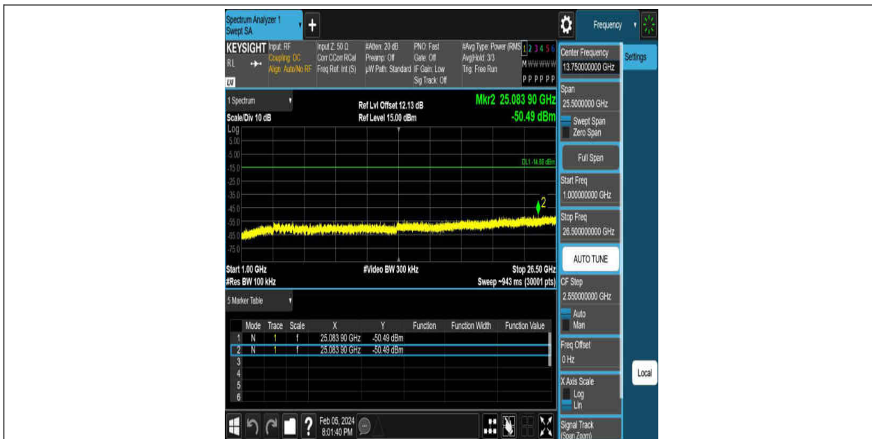
2DH5-Ant1-2441-1000~26500-PASS
