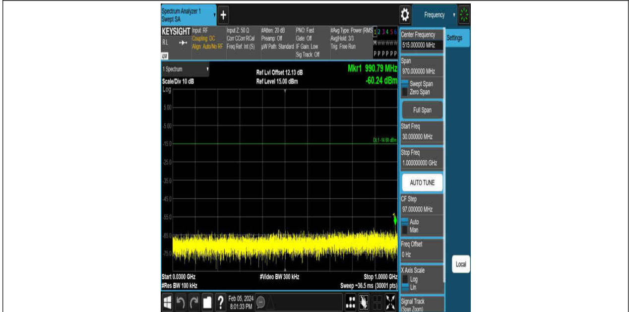
2DH5-Ant1-2441-30~1000-PASS
