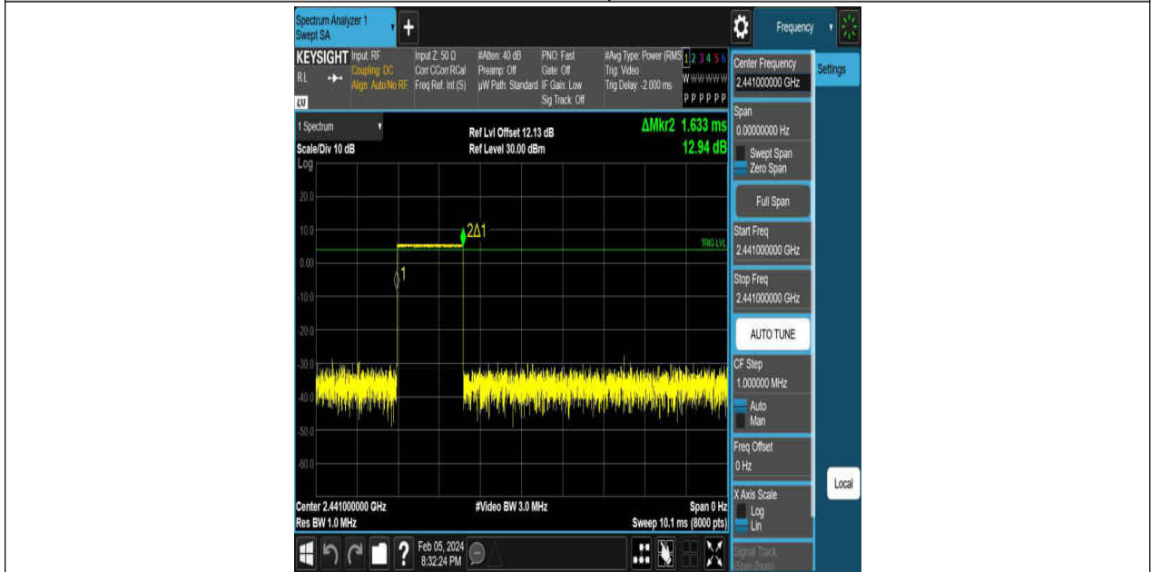
DH3-Ant1-Hop-PASS
