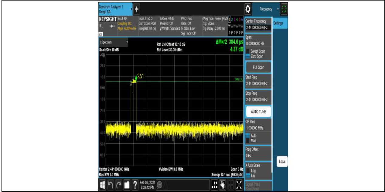
2DH1-Ant1-Hop-PASS
