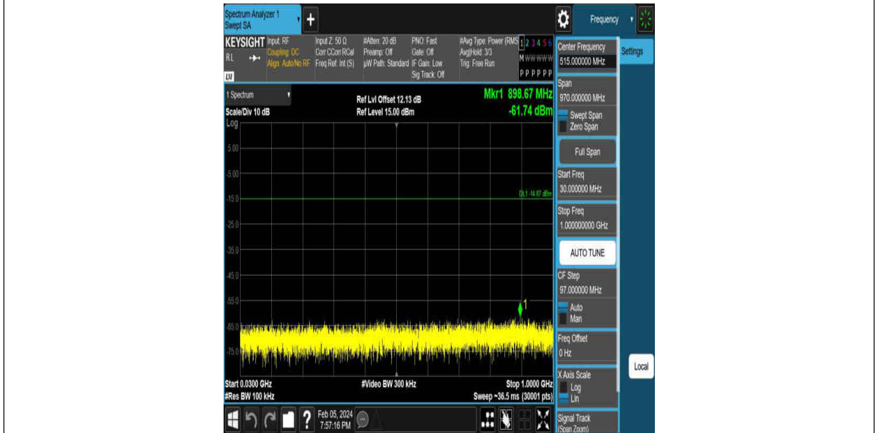
DH5-Ant1-2441-30~1000-PASS
