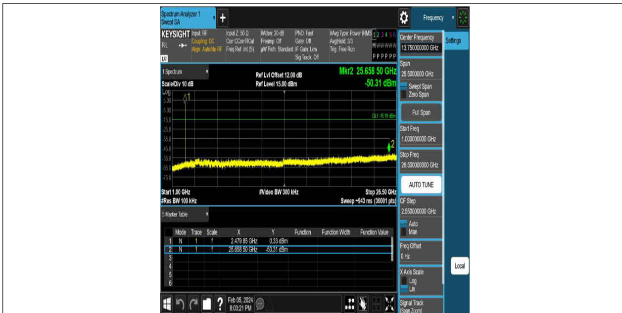
2DH5-Ant1-2480-1000~26500-PASS
