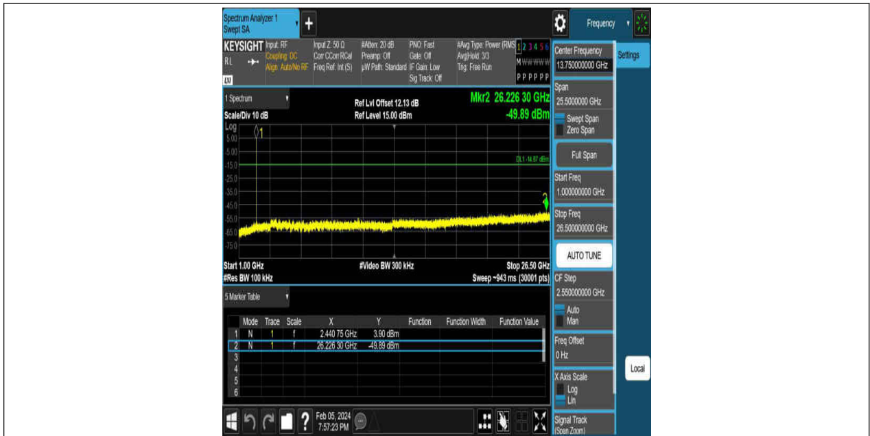
DH5-Ant1-2441-1000~26500-PASS
