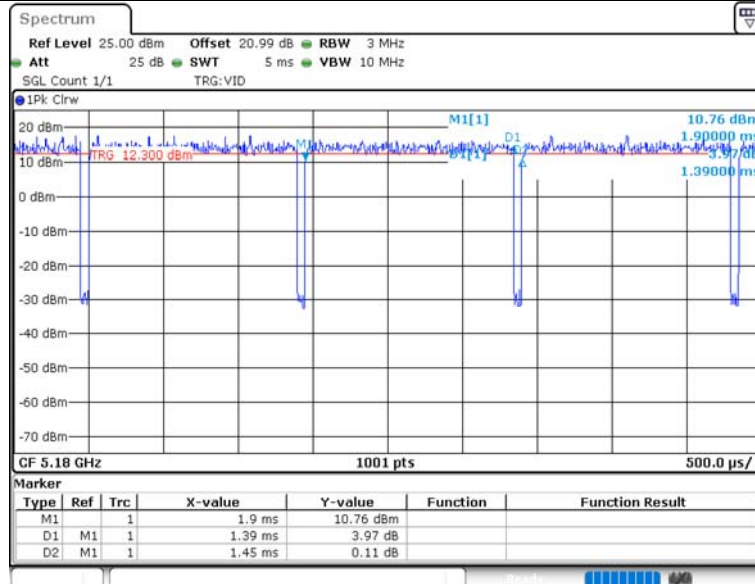
11A_Ant2_5180
