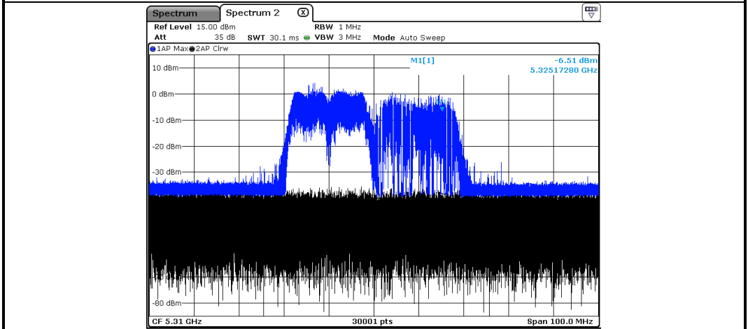
EUT (Client ) links with master on 5310MHz
