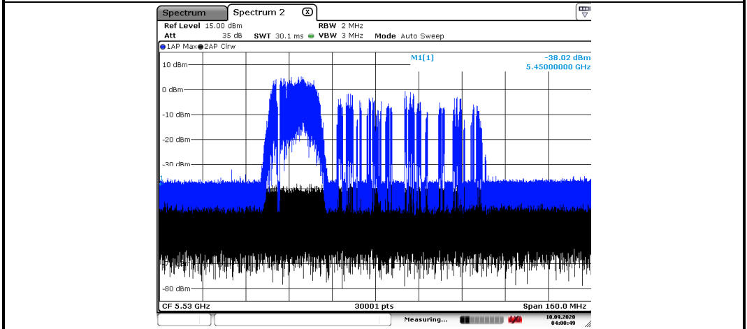
EUT (Client ) links with master on 5530MHz
