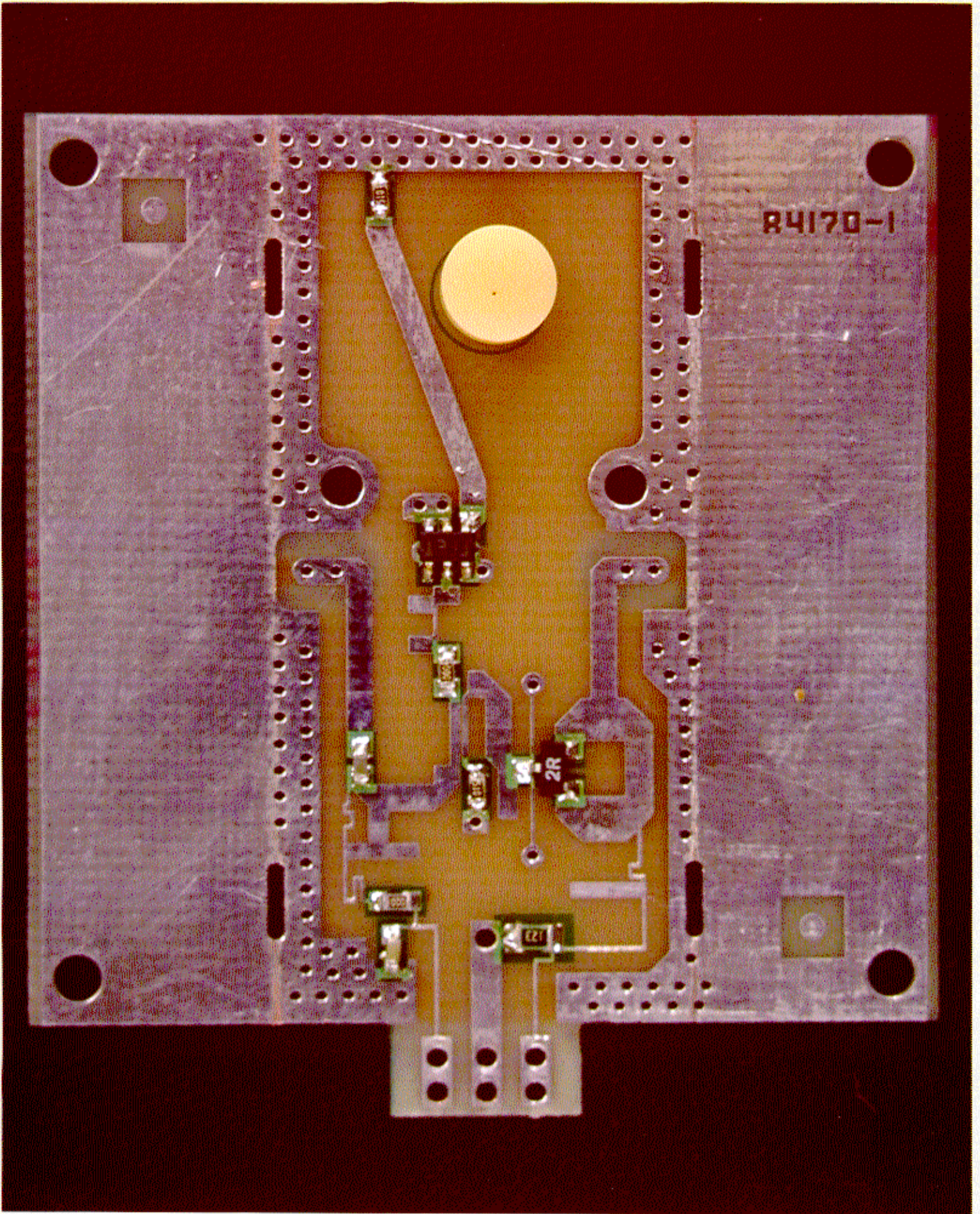
Photograph : NJR4170 (The inner circuits)
