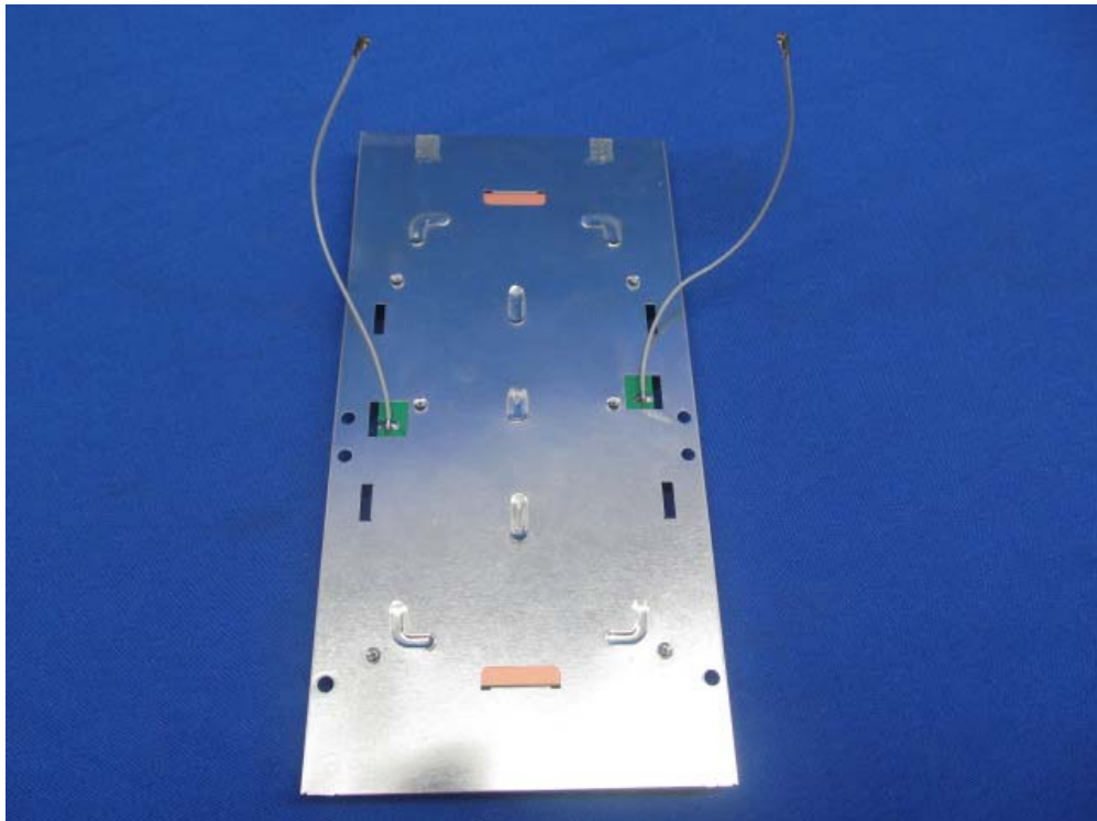
(4) EUT Photo (17dBi Antenna)
