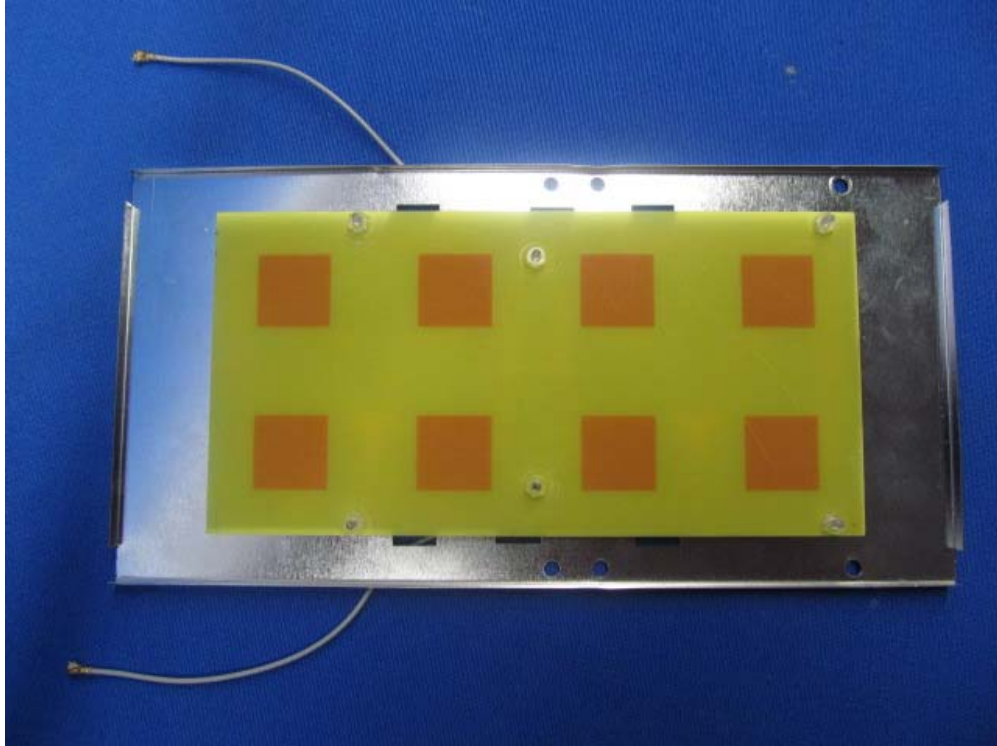
(3) EUT Photo (17dBi Antenna)
