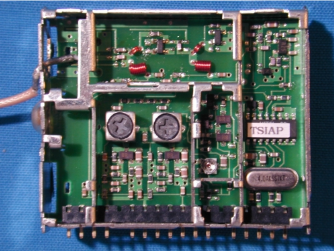
(7) EUT Photo
