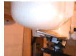
Figure 14.4 Right Head SAR Test Setup -- Ear / Tilt Position --
