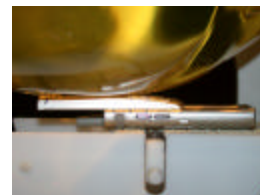
Figure A.2 Right Head SAR Test Setup -- Cheek / Touch Position – (Slider Out)
