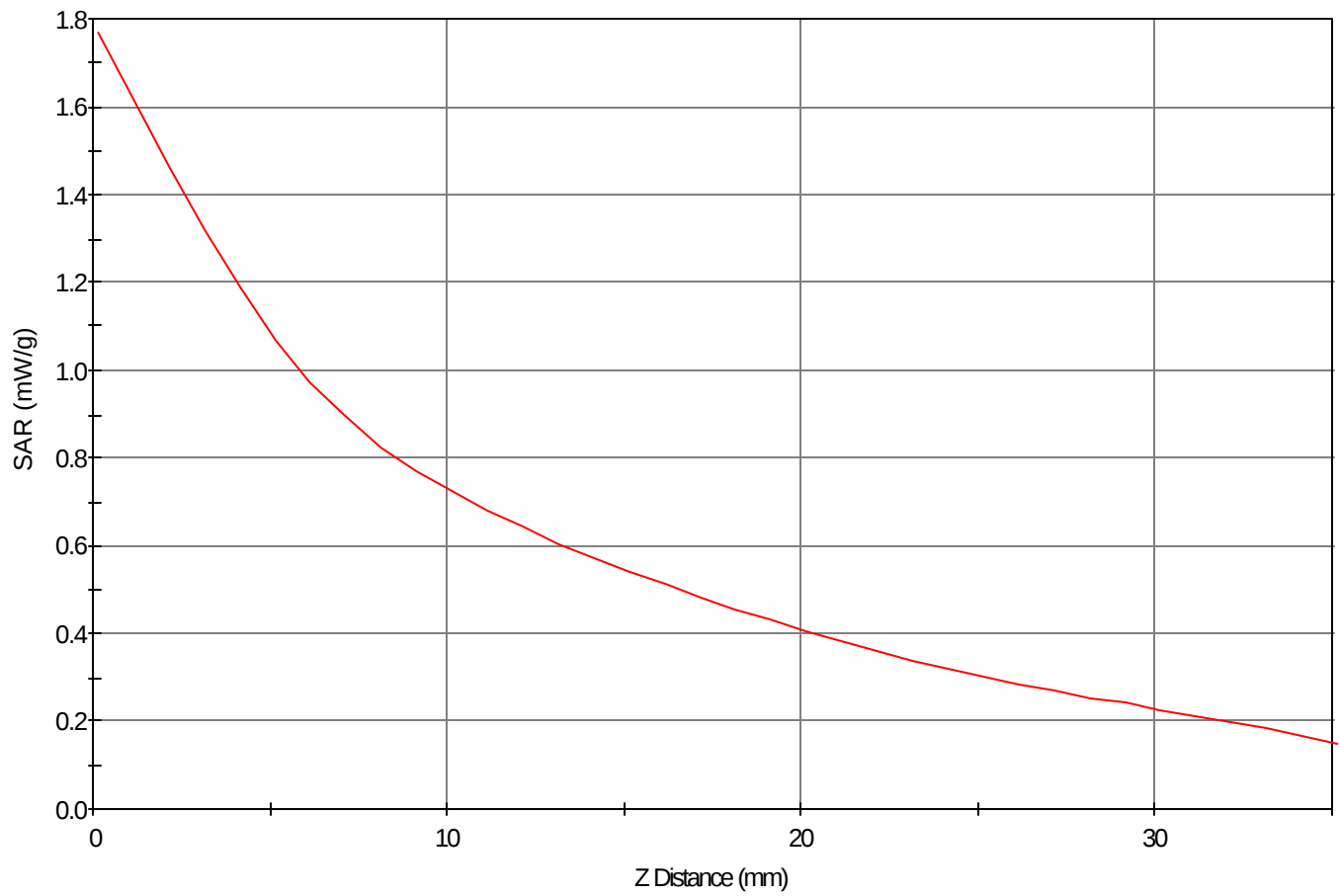
SAR - Z Axis at Hotspot x:9.0 y:-20.5
