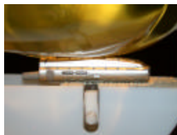
Figure A.1 Right Head SAR Test Setup -- Cheek / Touch Position – (Slider In)
