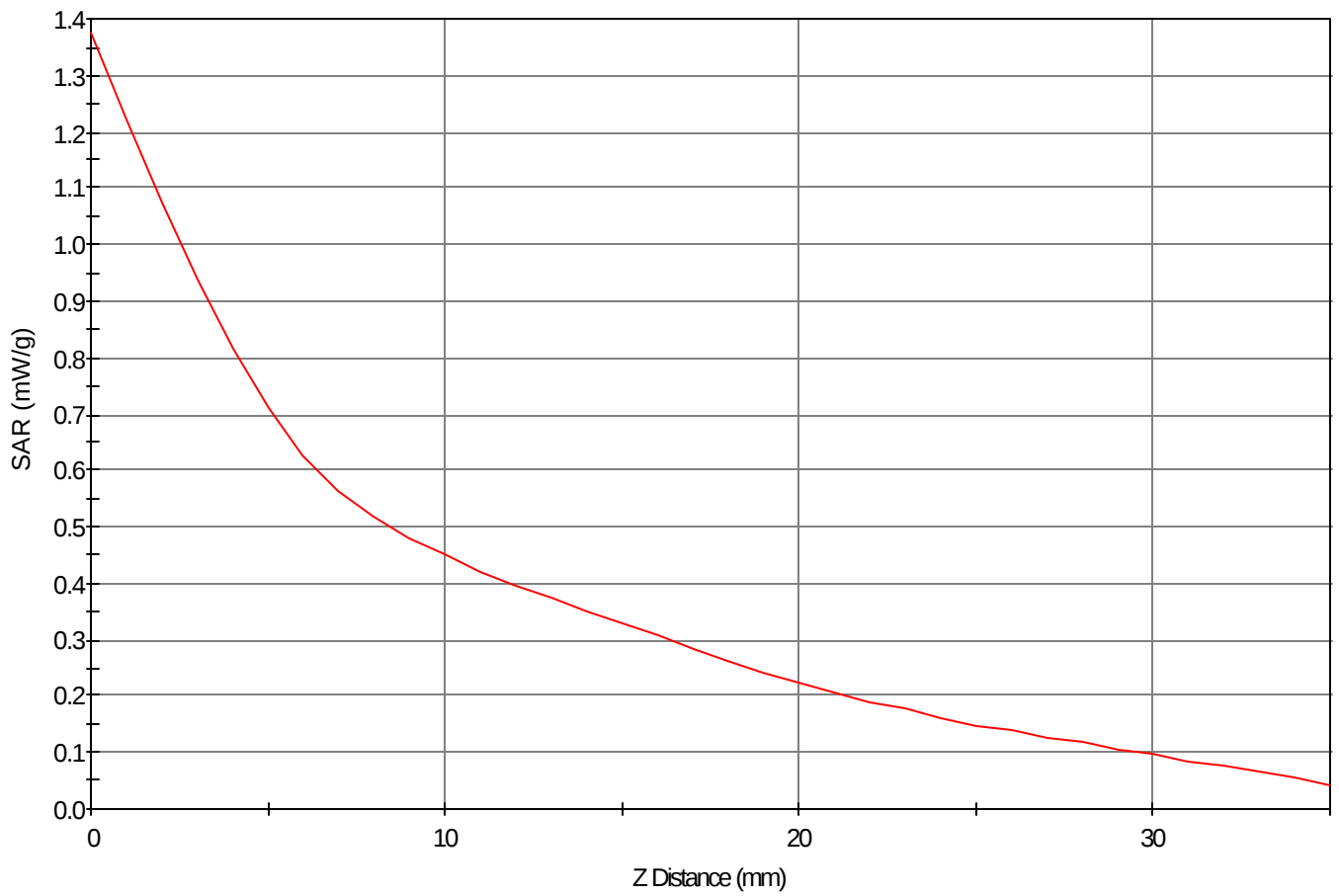
SAR - Z Axis at Hotspot x:-3.0 y:11.5
