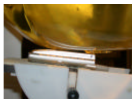
Figure A.5 Left Head SAR Test Setup -- Cheek / Touch Position -- (Slider In)
