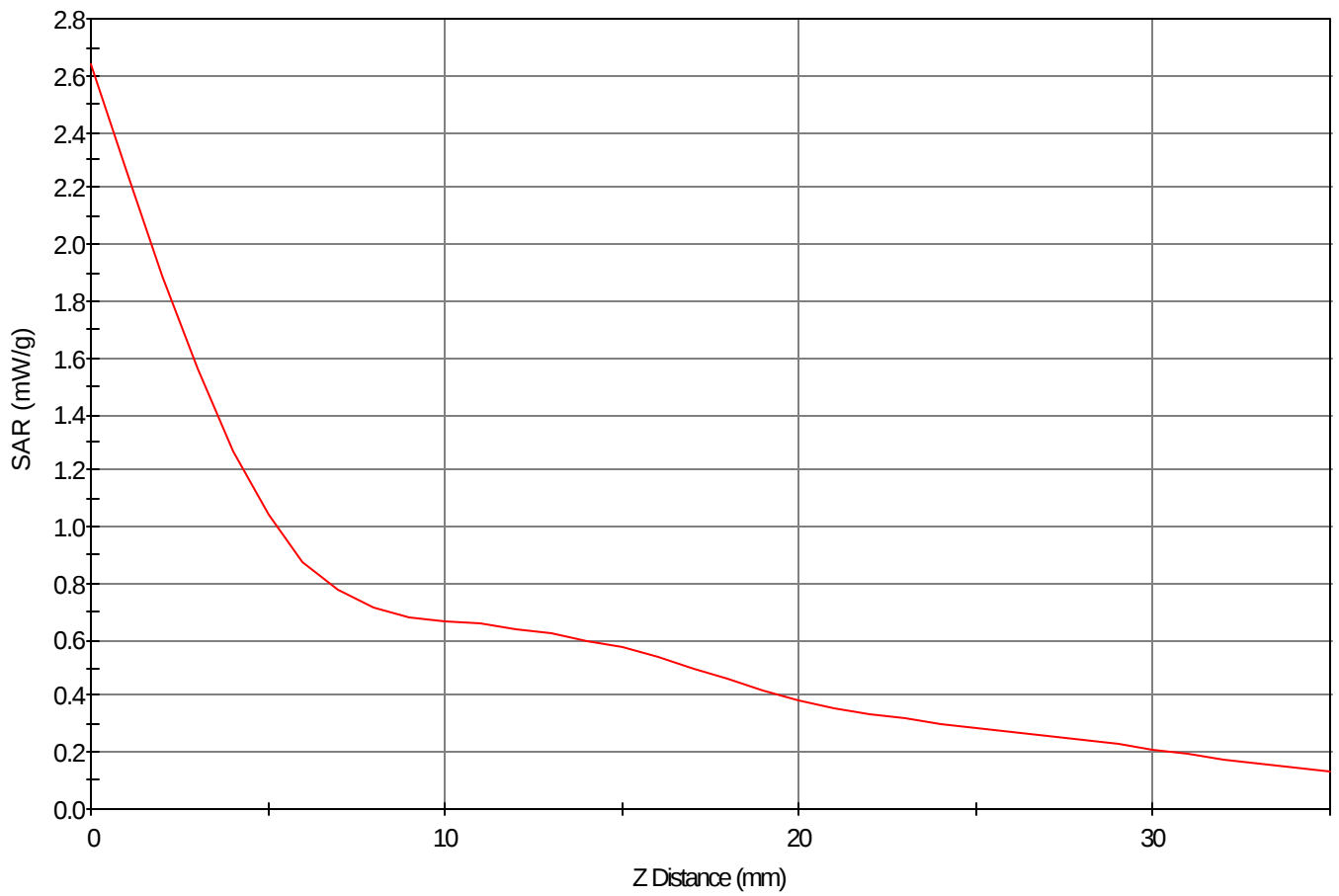
SAR - Z Axis at Hotspot x:34.0 y:-0.5
