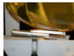
Figure A.6 Left Head SAR Test Setup -- Cheek / Touch Position -- (Slider Out)
