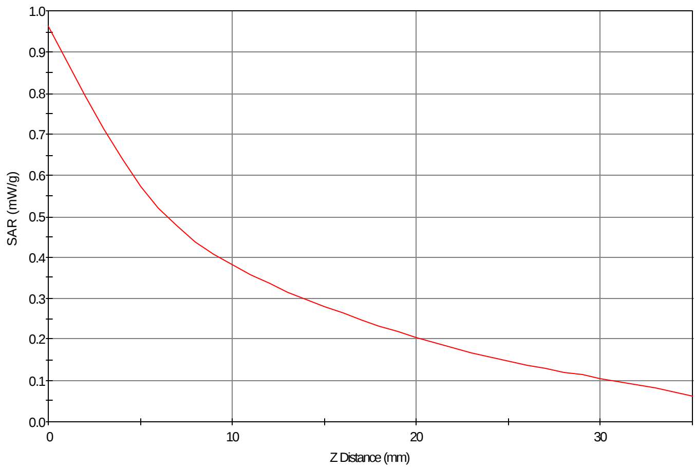
SAR - Z Axis at Hotspot x:-1.0 y:13.5
