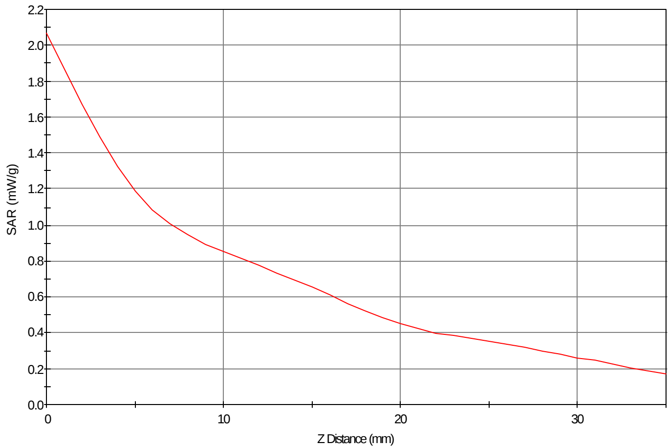
SAR - Z Axis at Hotspot x:18.0 y:-1.5
