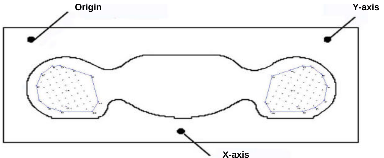
Fig 10. SAR Measurement Points in Area Scan
