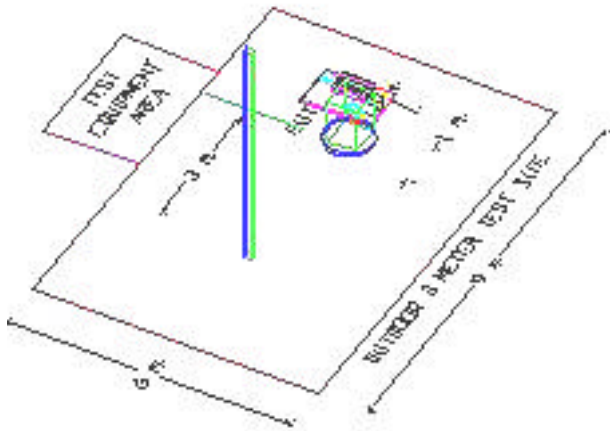
Figure 2. Turntable, Antenna mast, and Test Setup
