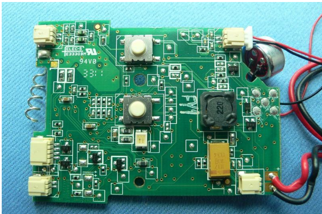
PCB Backside
