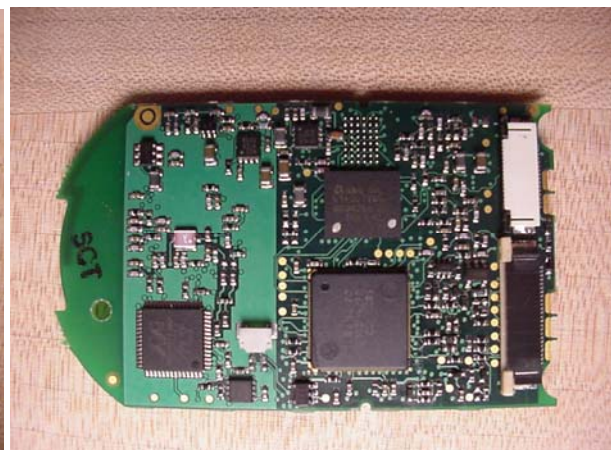
Mobile IPTouch 300 RF Generation Board – Side B
