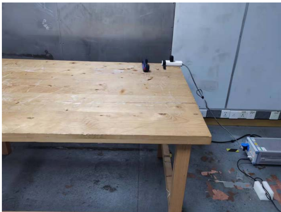
Photo of Power Line Conducted Emission Measurement - Front View Adapter Charging
