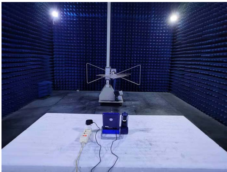
Photo of Radiated Emission Measurement Below 1GHz Telephone Base Charging
