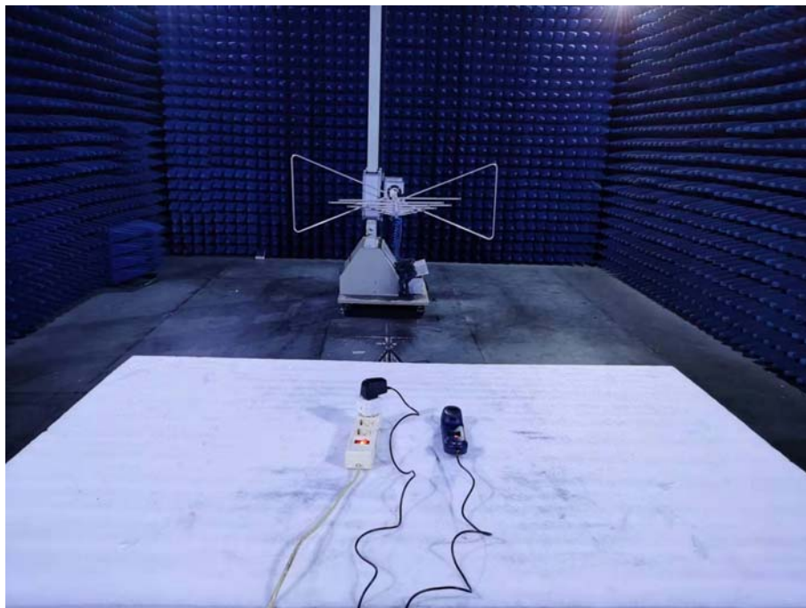
Photo of Radiated Emission Measurement Below 1GHz Adapter Charging
