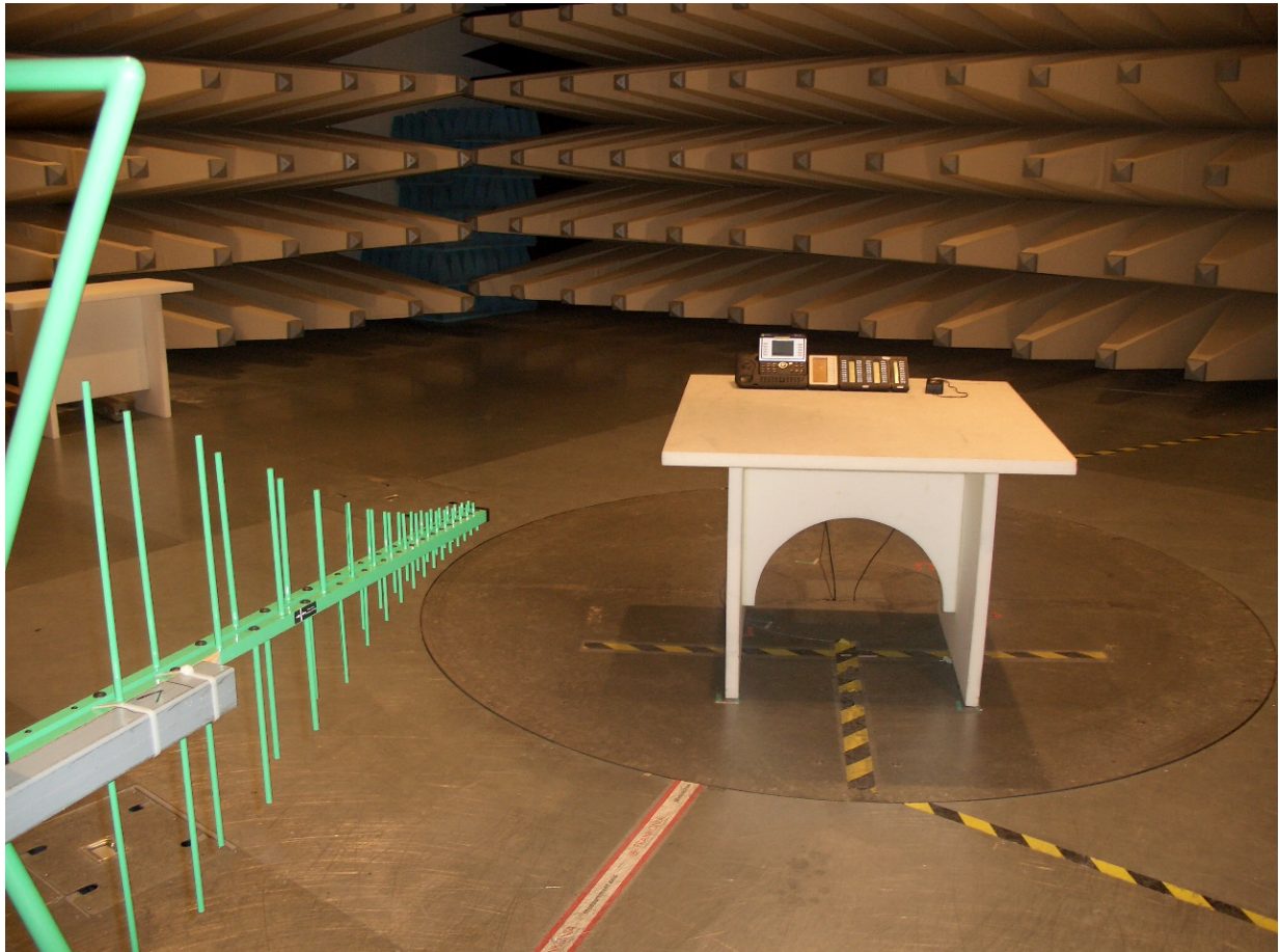
Photo 1: Radiated Emissions
