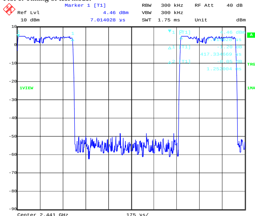
Plot 1: Timing of test mode:
