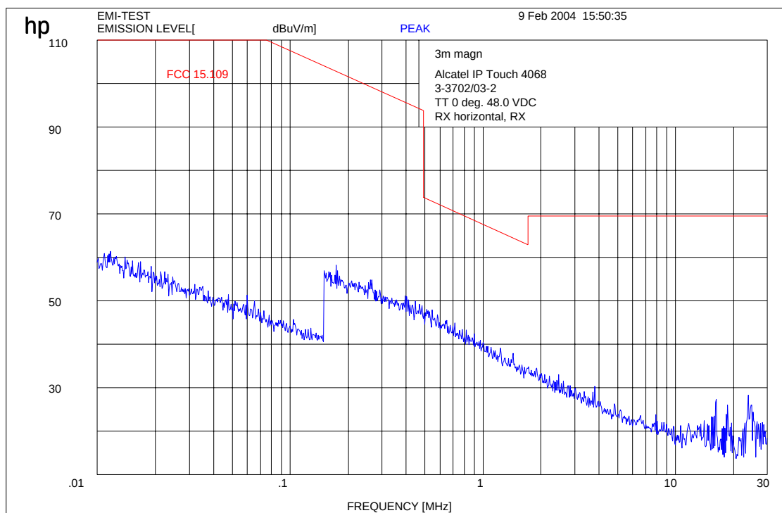
Plot 2: RX Mode
