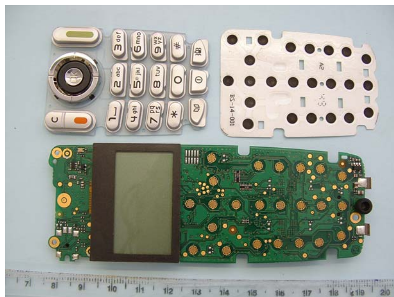
MR300 PCB KEYPAD SIDE KEY COVER REMOVED
