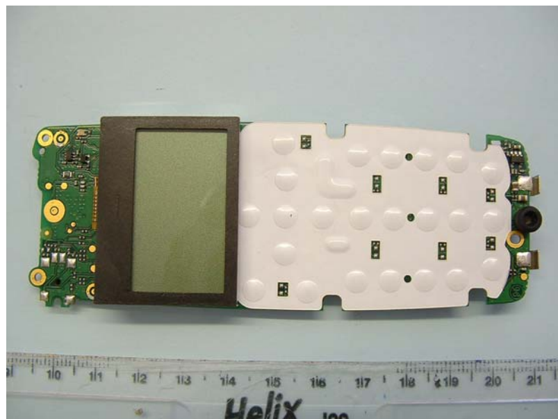
MR300 PCB KEYPAD SIDE
