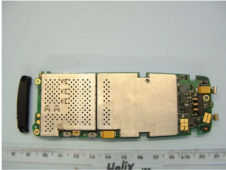
MR300 ASSEMBLED PCB RF SIDE
