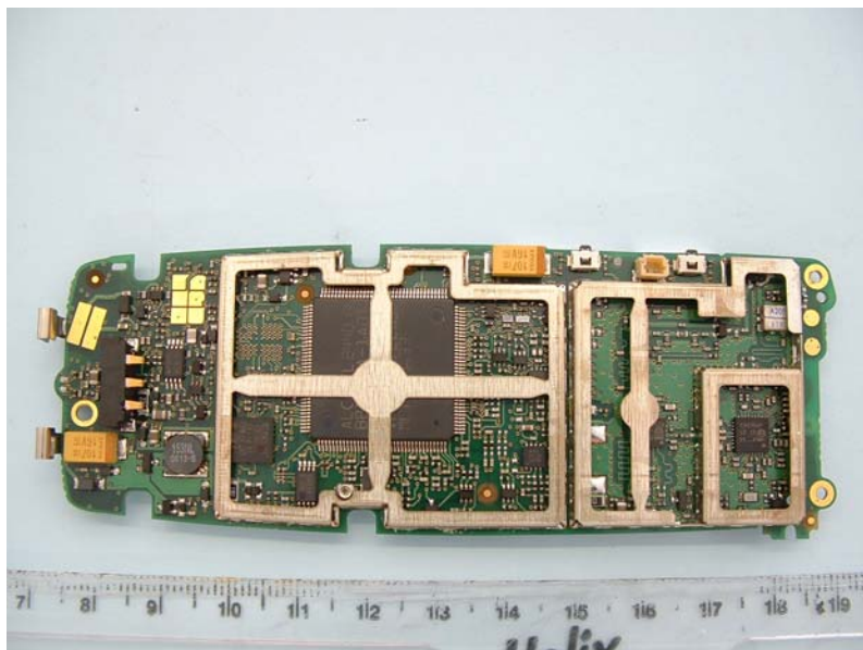
MR300 PCB RF SIDE CANS REMOVED
