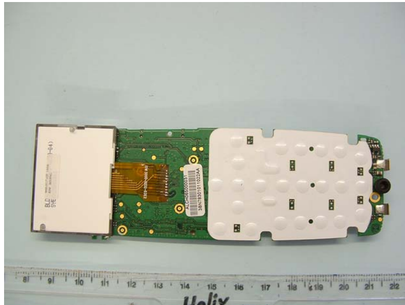
MR300 PCB KEYPAD SIDE LCD MOVED
