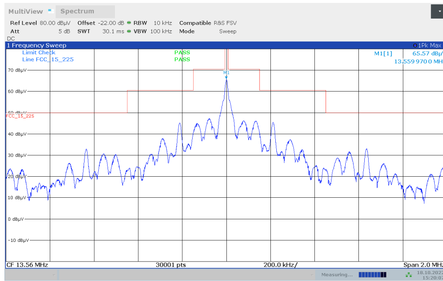
Plot 3: Spectrum mask (the limits are recalculated according to the ANSI C63.10-2013 sub clause 6.4)
