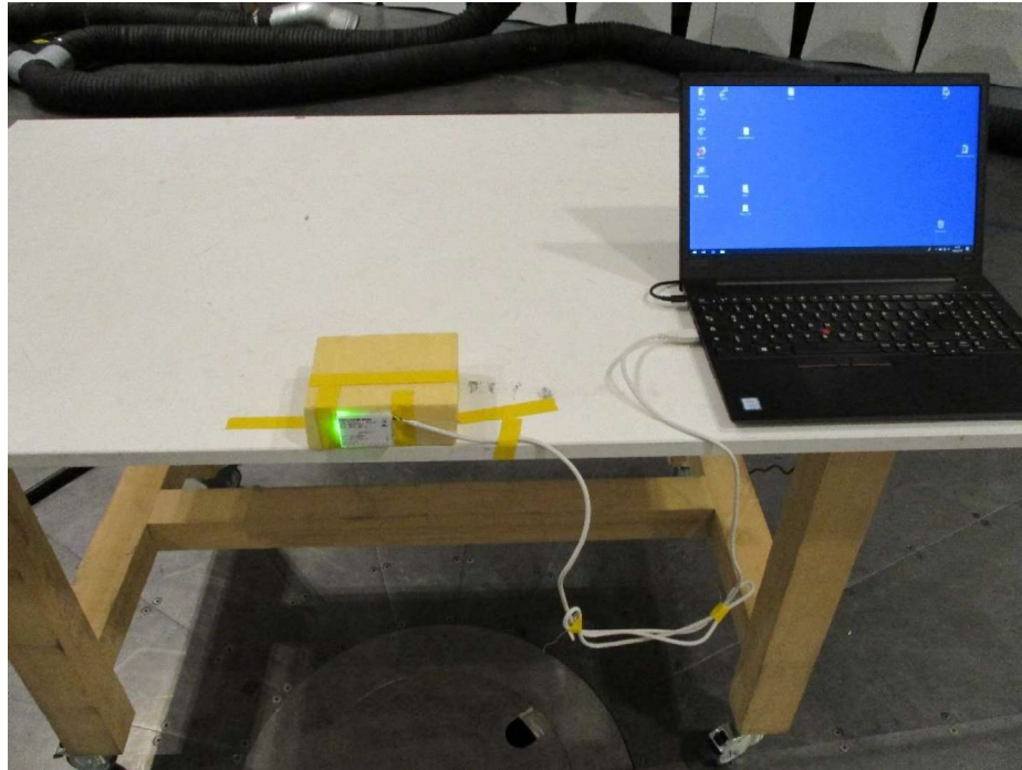
Figure 10 - Test setup for radiated emission
