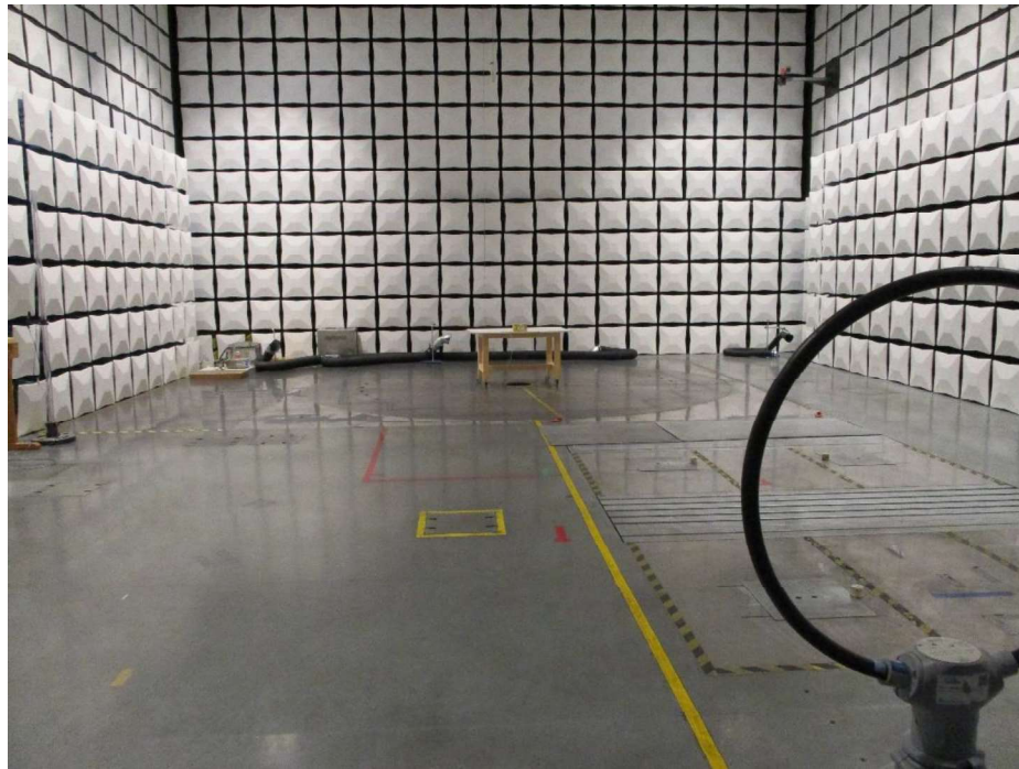
Figure 12 - Test setup for radiated emission 9kHz-30M
