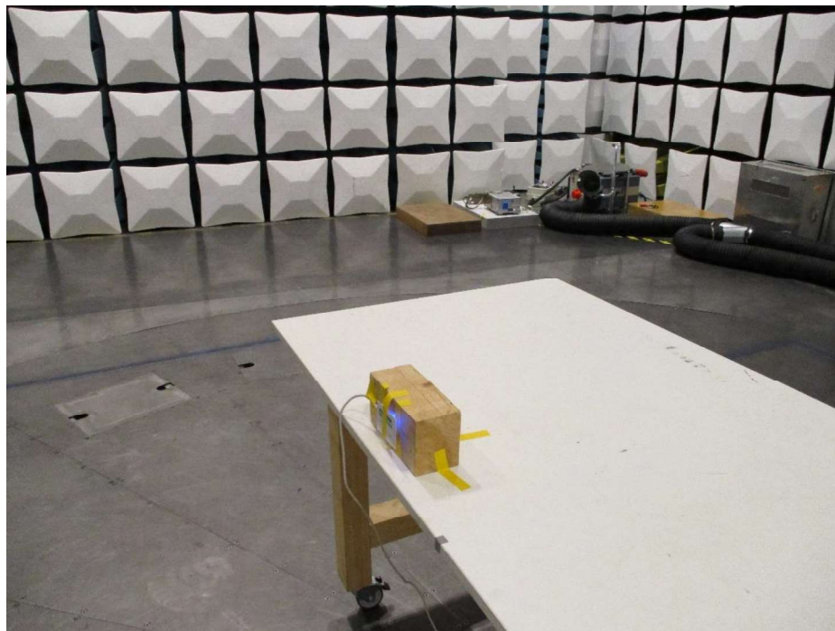
Figure 13 - Test setup for radiated emission 9kHz-30MHz
