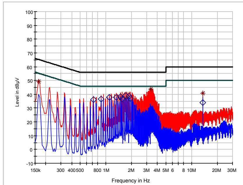
— FCC § 15.207 QP — FCC § 15.207 AV — Preview Result 1-PK+ * Final Result 1-QPK ◇ Preview Result 2-AVG ◇ Final Result 2-AVG
