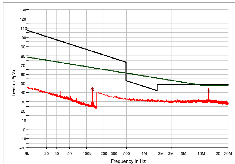
K8 CISPR 16-2-3 Magnetic Field Strength 9kHz - 30 MHz
