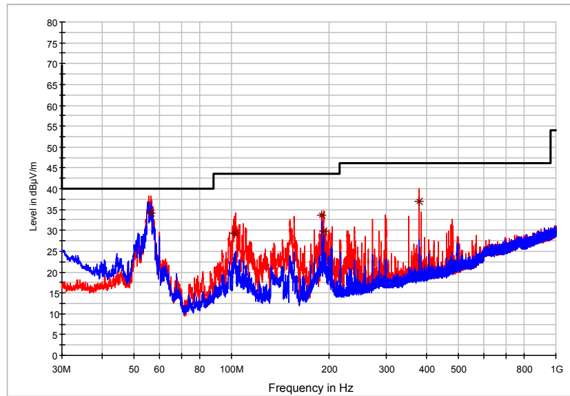
K8 CISPR 16-2-3 Electric Field Strength 30MHz-1GHz (3m)
