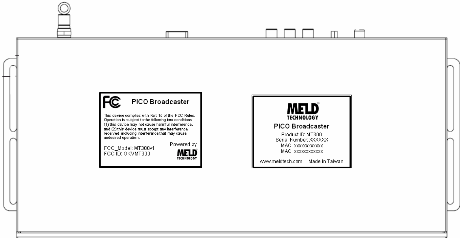
Bottom view of device (drawing not exactly to scale)
