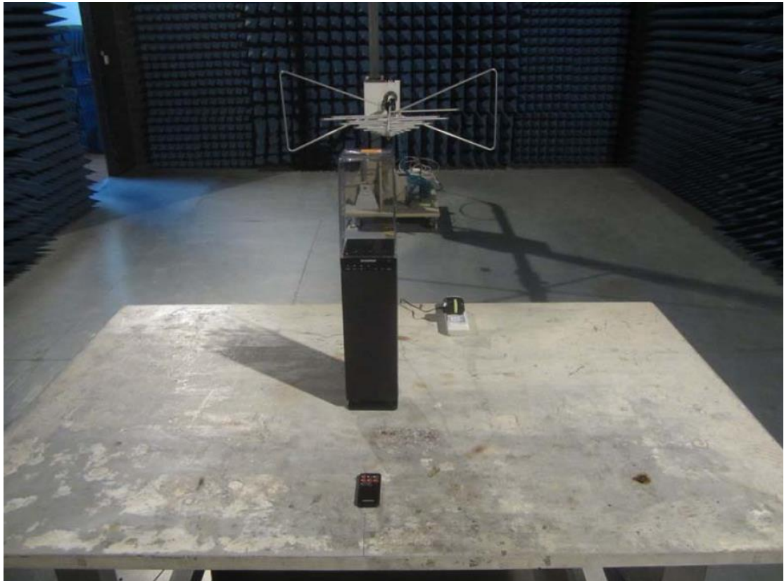
Radiated emission:
