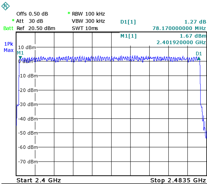
Modulation: 8DPSK
