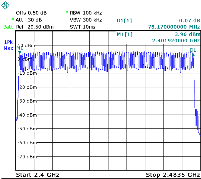
Modulation: GFSK
