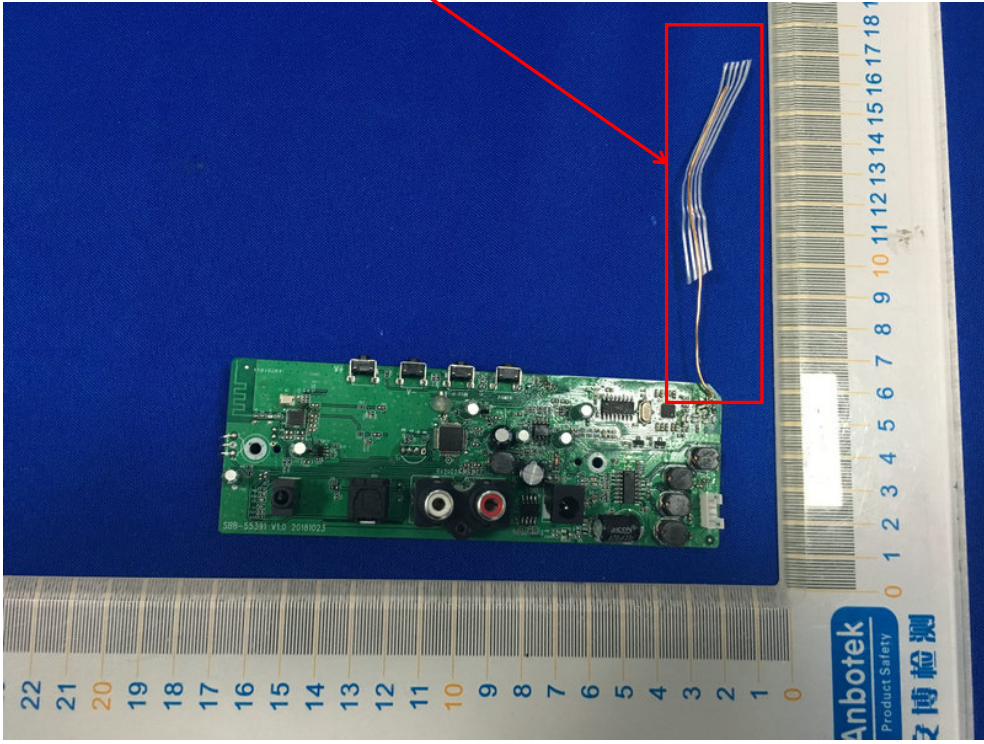
Wire Antenna
