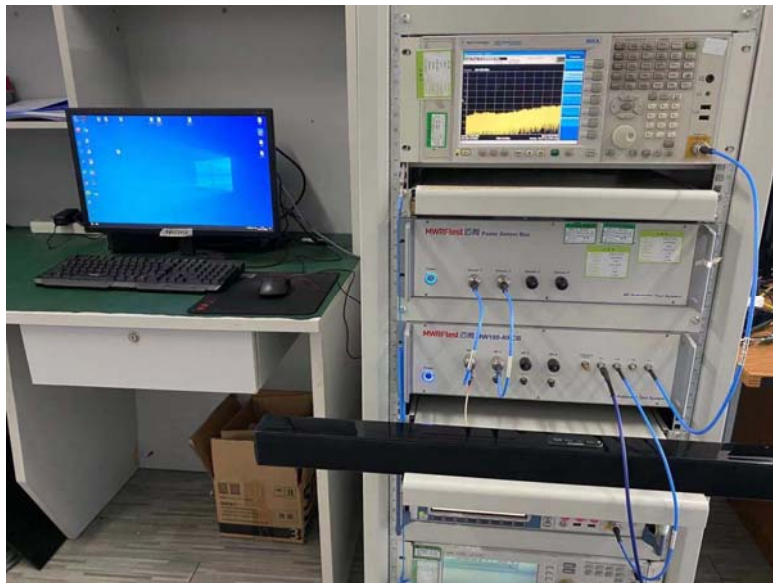
Conducted RF
