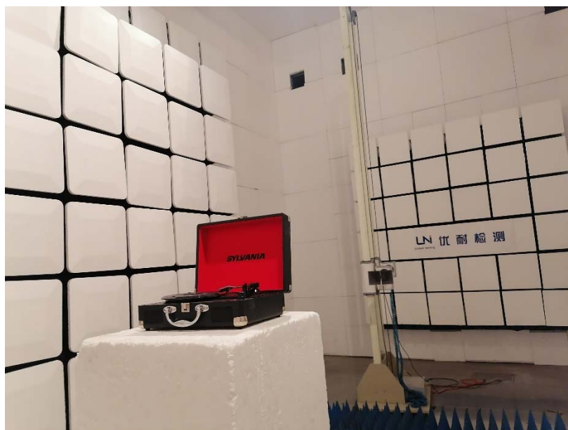
Radiated Emission Photo 2
