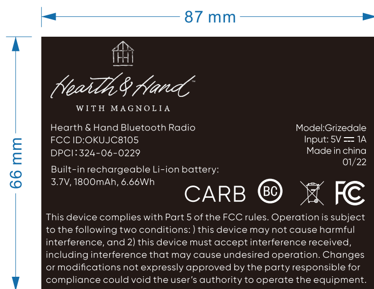
[1] Rating Label
