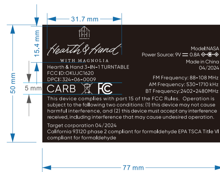
[1] Rating Label
