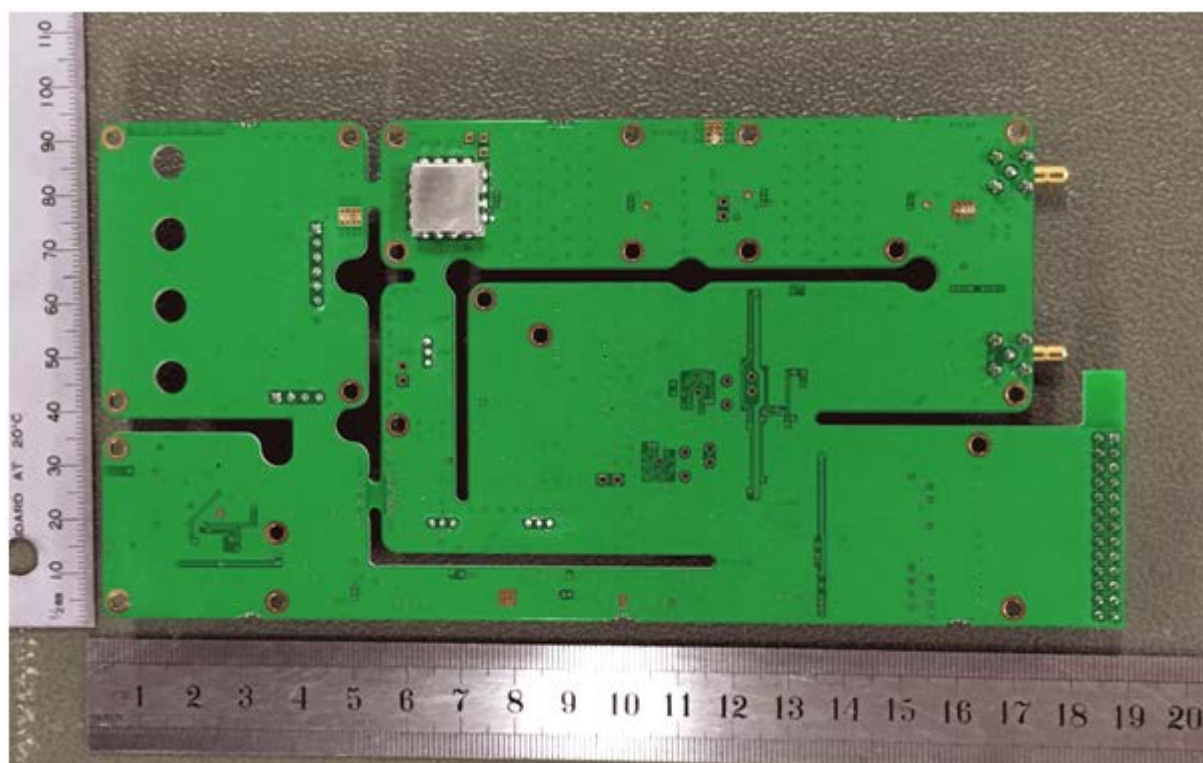
Figure 10. Receiver PCB Bottom View.
