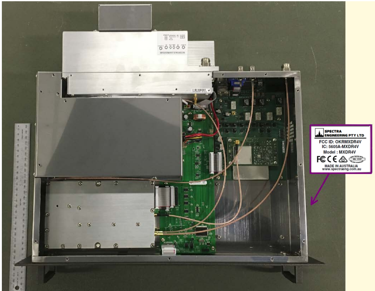
Figure 27 FCC ID LABEL LOCATION- View
